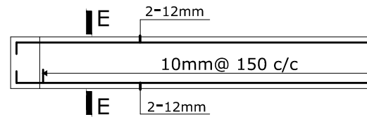
R.c Lintel details
