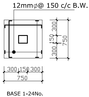
R.C Column base detail
